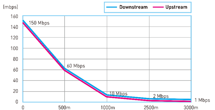
Symmetric Profile Data Rate (over 26AWG)
